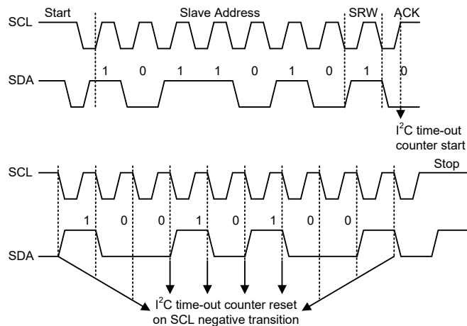
I²C Time-out
