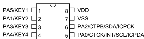
BS83A04C 8 SOP-A
