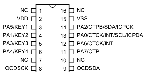
BS83AV04C 16 NSOP-A
