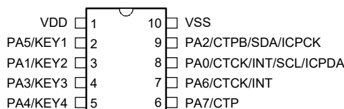
BS83A04C 10 DFN-A/MSOP-A
