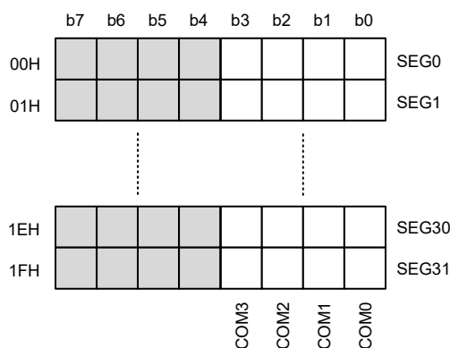
LCD Memory Map
