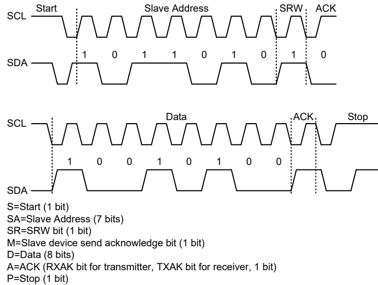
I²C Communication Timing Diagram
