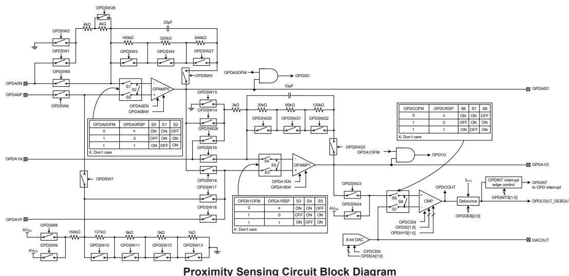
Proximity Sensing Circuit Block Diagram
