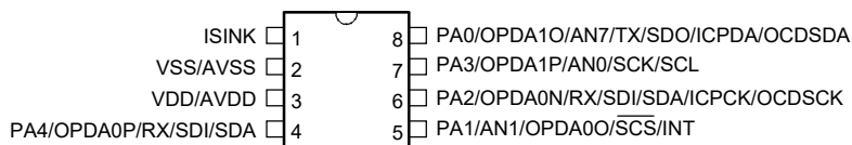
BS45F3232/BS45V3232 8 SOP-A
