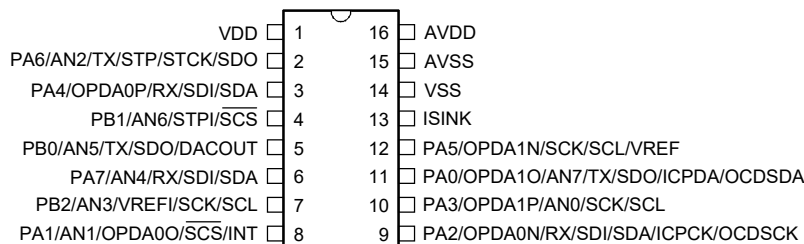
BS45F3232/BS45V3232 16 NSOP-A
