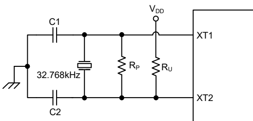
External LXT Oscillator
