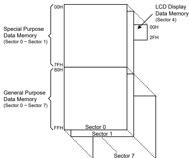
Data Memory Structure
