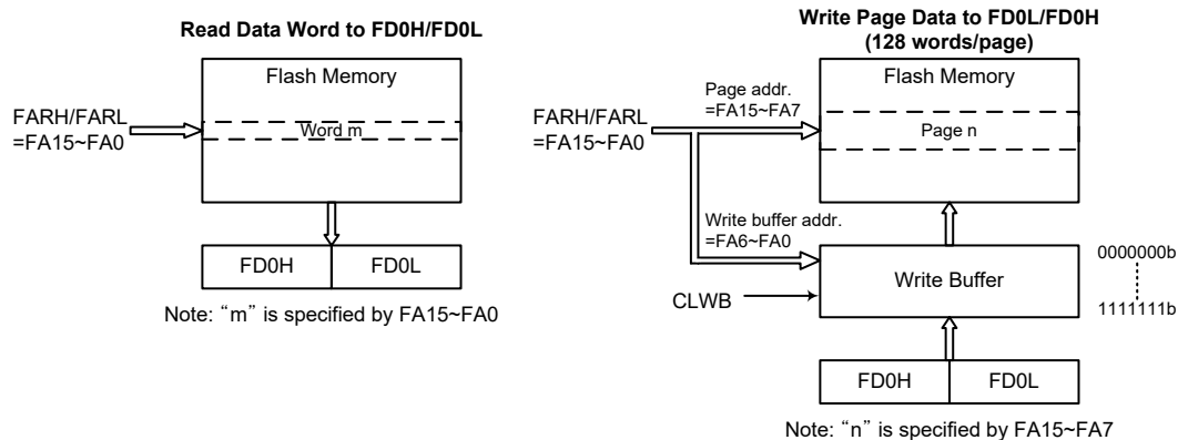
Flash Memory IAP Read/Write Structure
