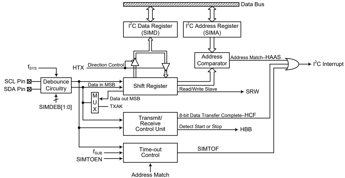
I²C Interface Block Diagram
