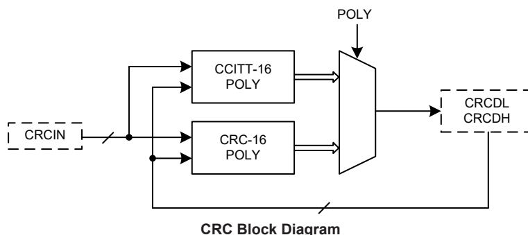
CRC Block Diagram
