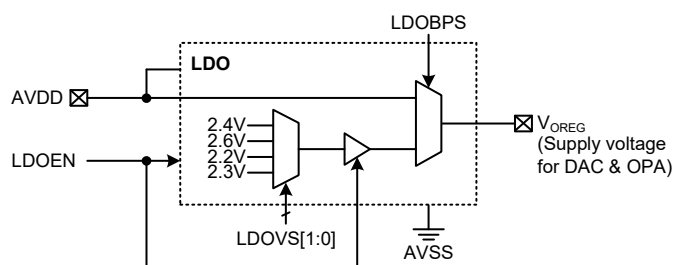
Internal Power Supply Block Diagram
