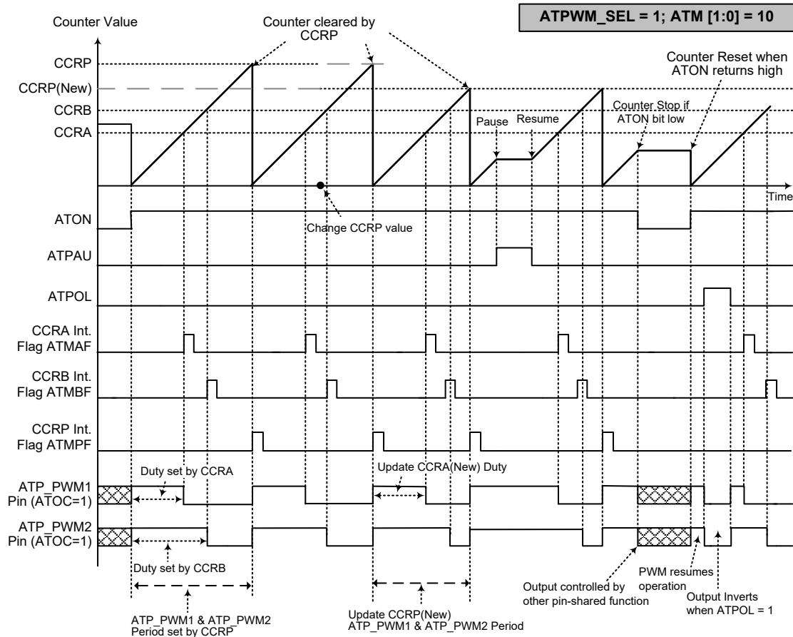
ATM Audio PWM Output Mode – Change CCRP Value
