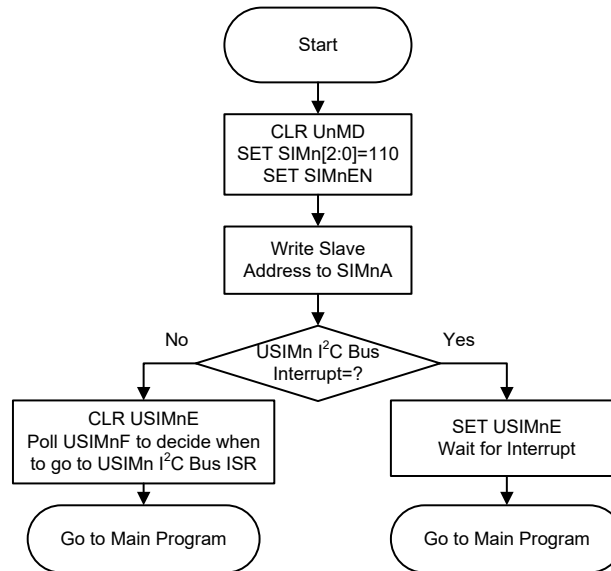
USIMn I 2 C Bus Initialisation Flow Chart
