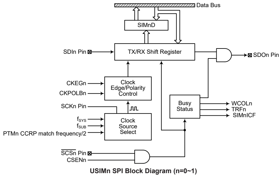
USIMn SPI Block Diagram (n=0~1)
