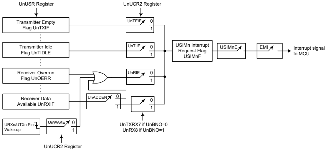
USIMn UART Interrupt Structure
