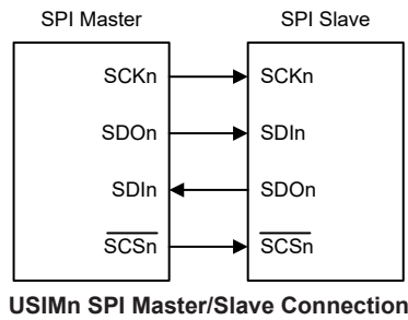
USIMn SPI Master/Slave Connection
