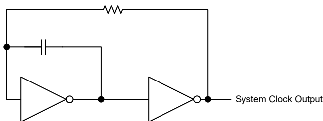
System Clock Oscillator
