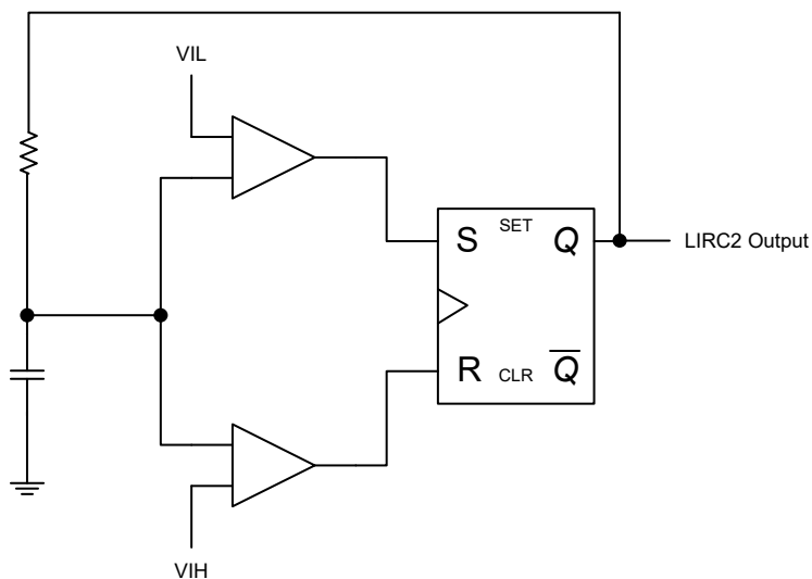
LIRC2 Oscillator
