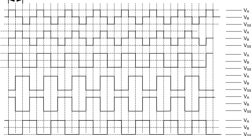
LCD Driver Output – Type B, 1/2 Duty, 1/2 Bias
