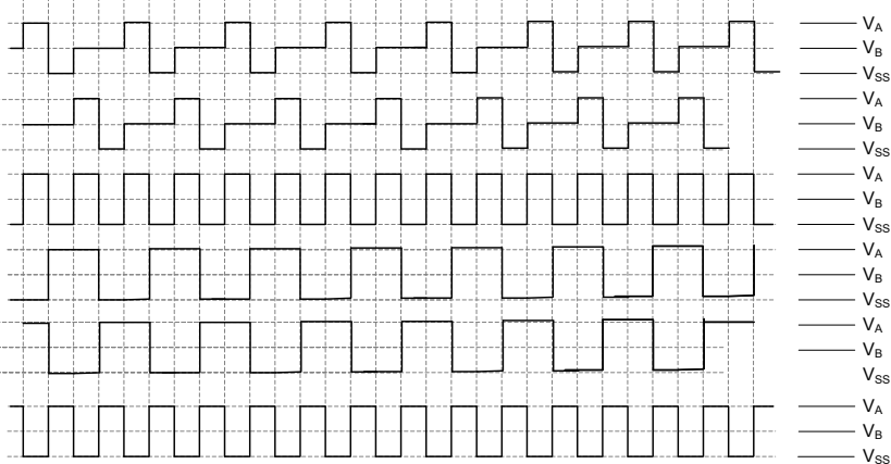
LCD Driver Output – Type A, 1/2 Duty, 1/2 Bias
