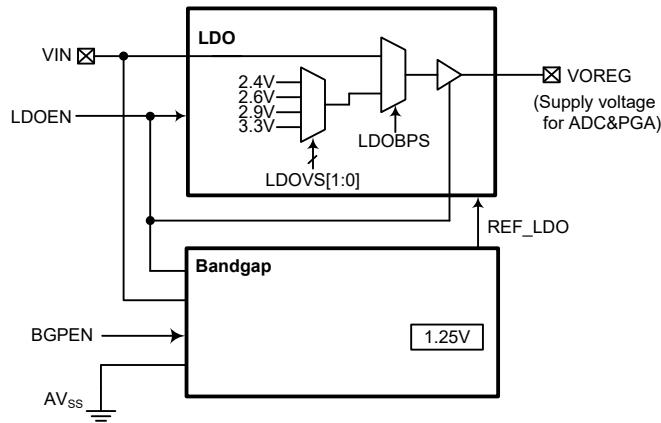
Internal Power Supply Block Diagram
