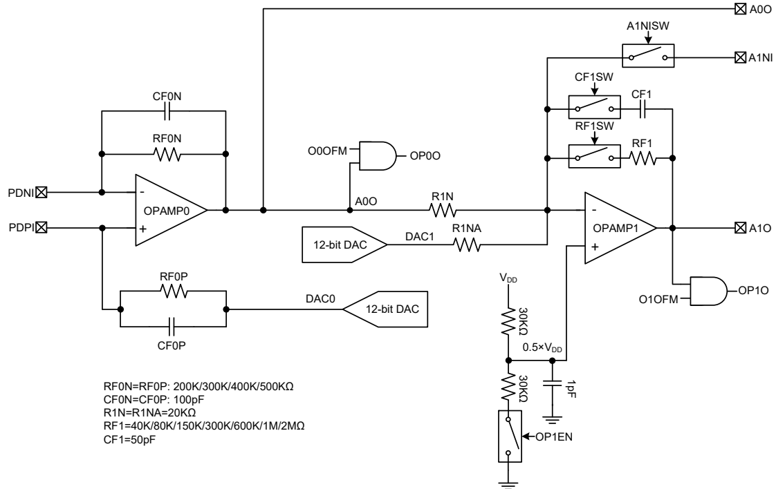
Pulse Oximeter AFE Block Diagram
