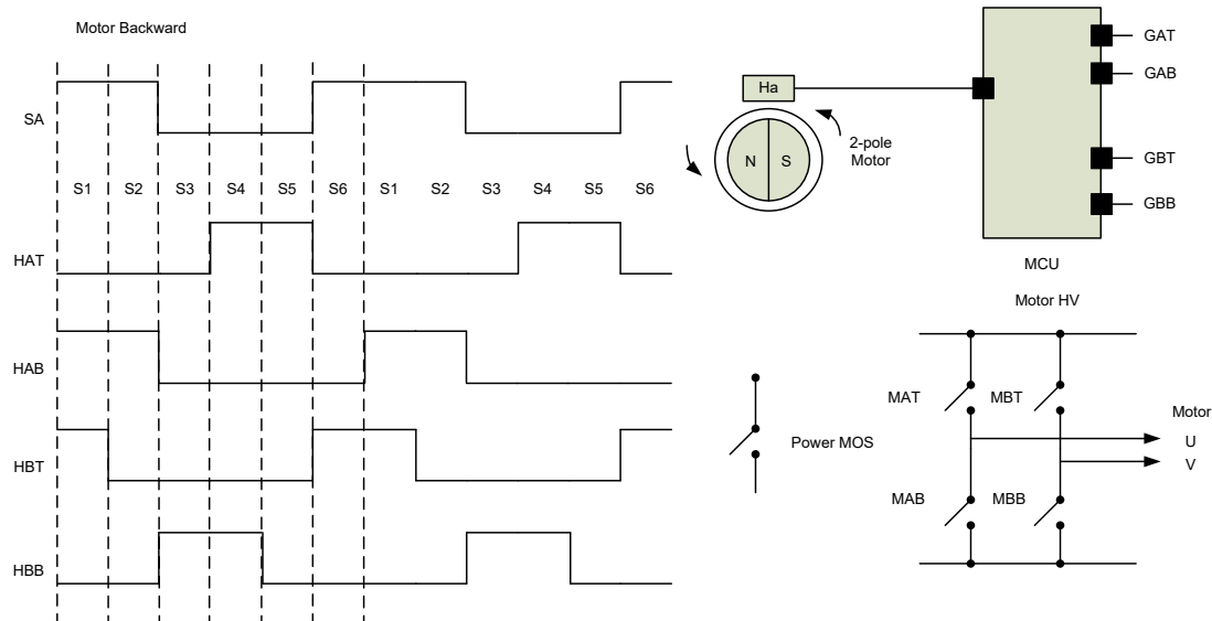
Motor Drive Signal Timing Diagram – Backward Direction
