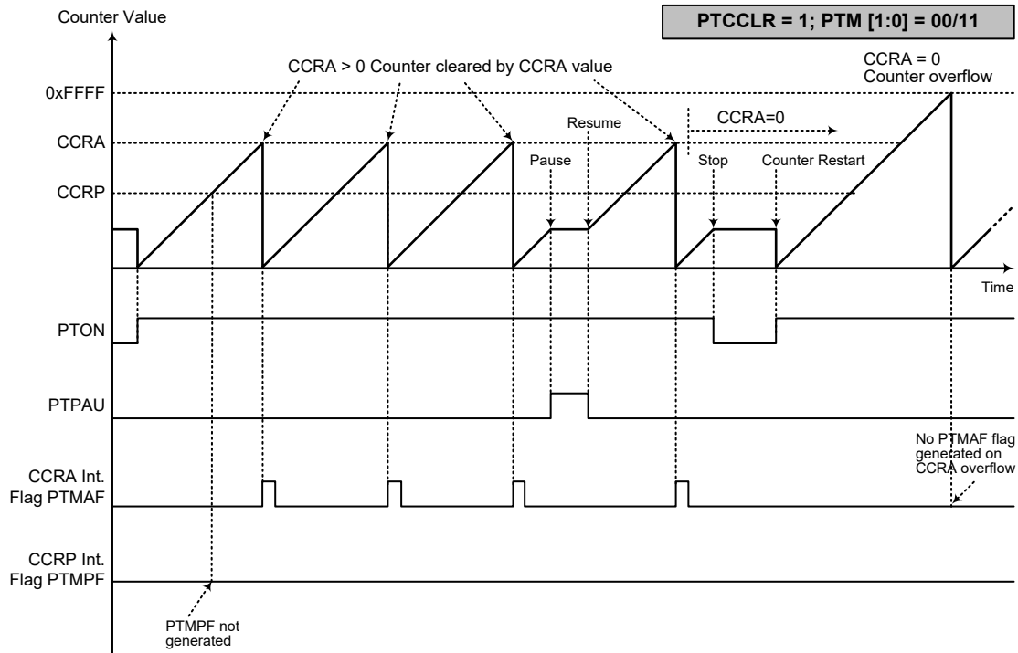
Timer/Counter Mode – PTCCLR=1
