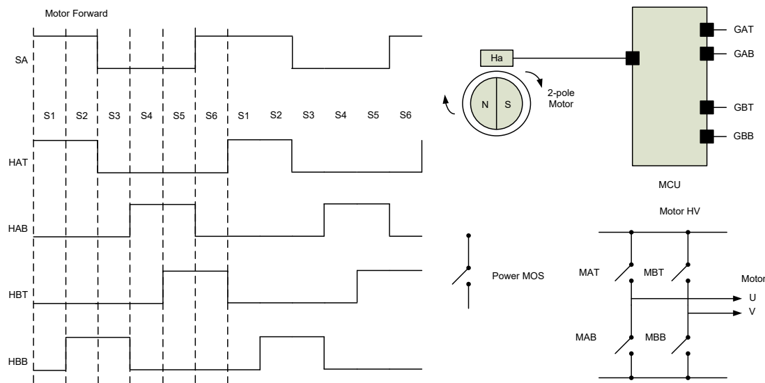
Motor Drive Signal Timing Diagram – Forward Direction
