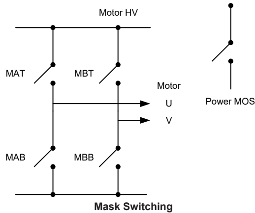
Mask Function Block Diagram
