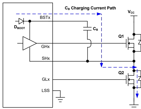
Bootstrap Capacitor ( C_B ) Charging Current Path
