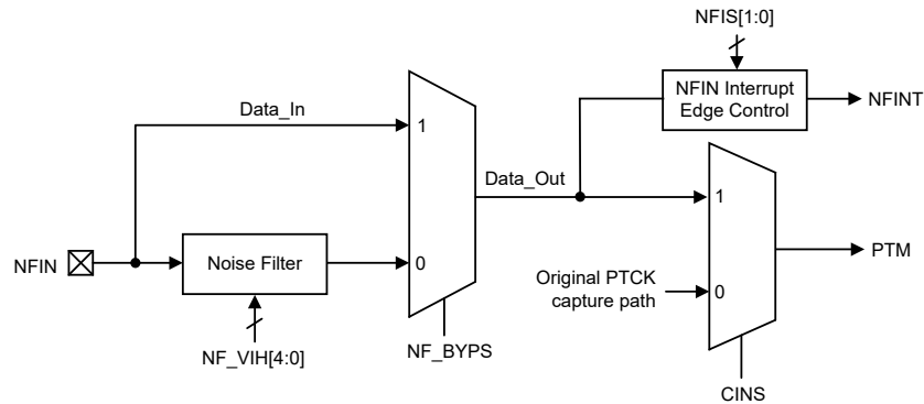
Digital Noise Filter Block Diagram
