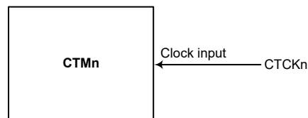
CTMn Function Pin Block Diagram (n=2)
