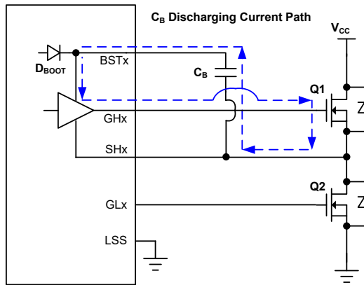
Bootstrap Capacitor ( C_B ) Discharging Current Path
