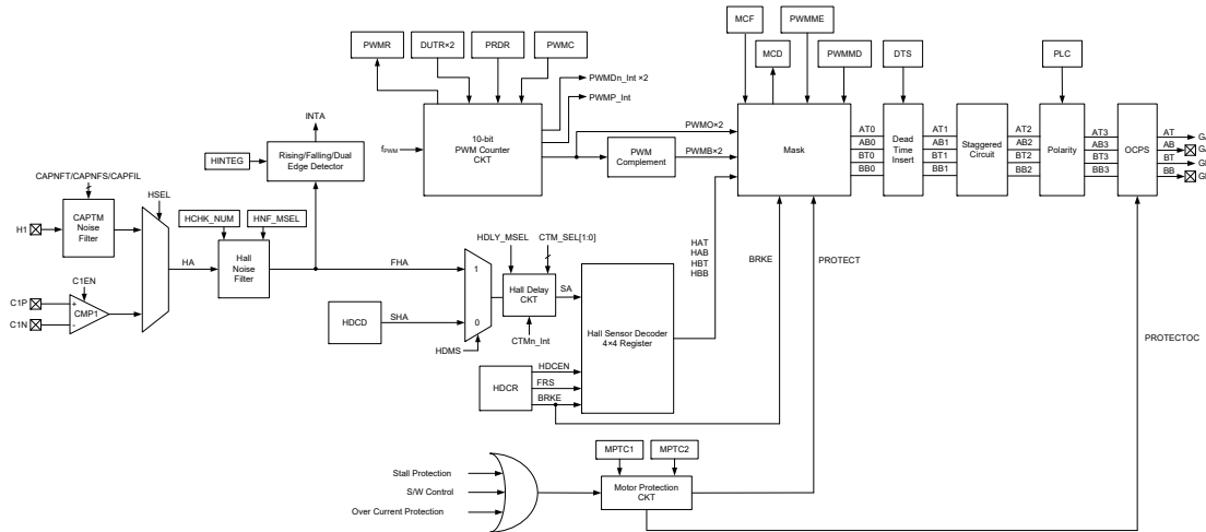
BLDC Motor Control Block Diagram
