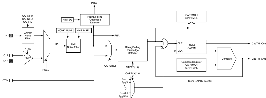
Capture Timer Block Diagram
