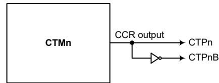
CTMn Function Pin Block Diagram (n=0~1)
