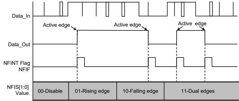
Digital Noise Filter Interrupt Trigger
