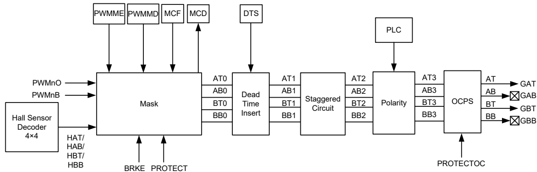
Mask Function Block Diagram
