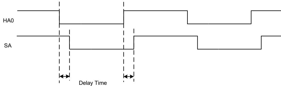
Delay Function Timing
