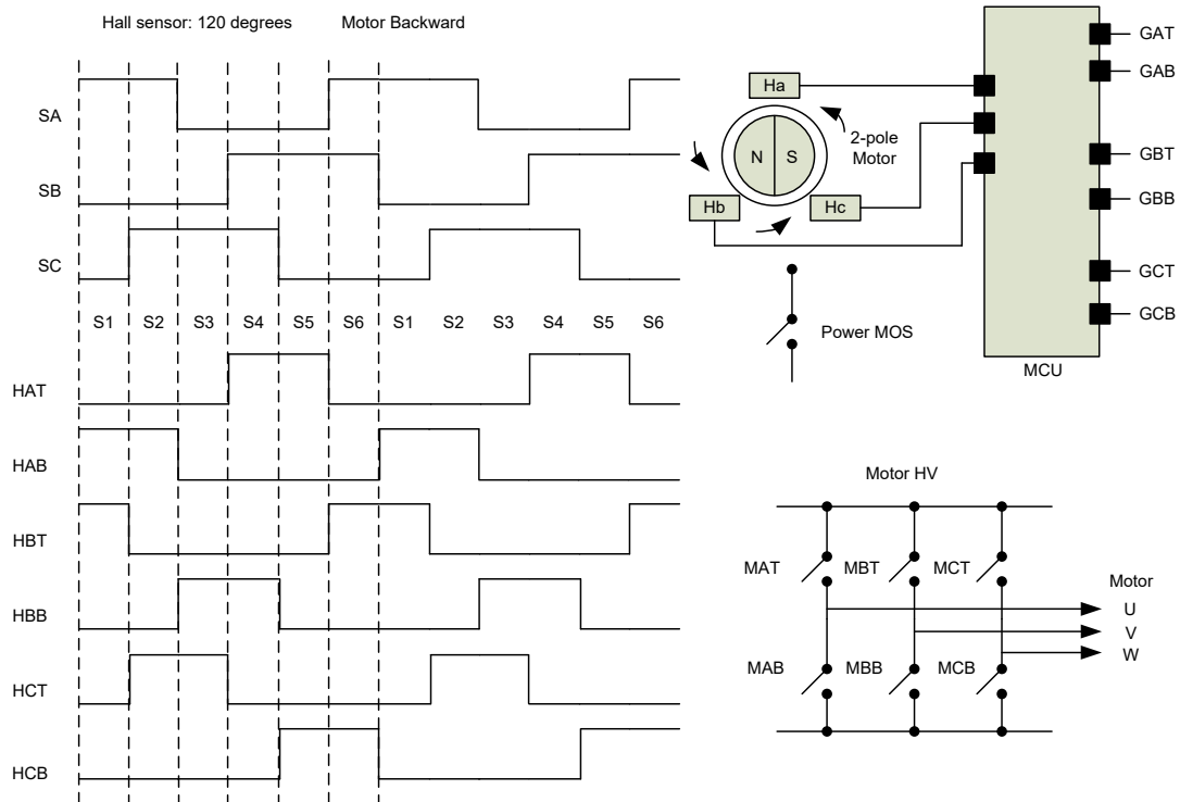
Motor Drive Signal Timing Diagram – Backward Direction
