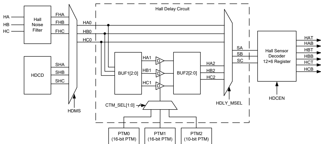
Hall Delay Function Block Diagram
