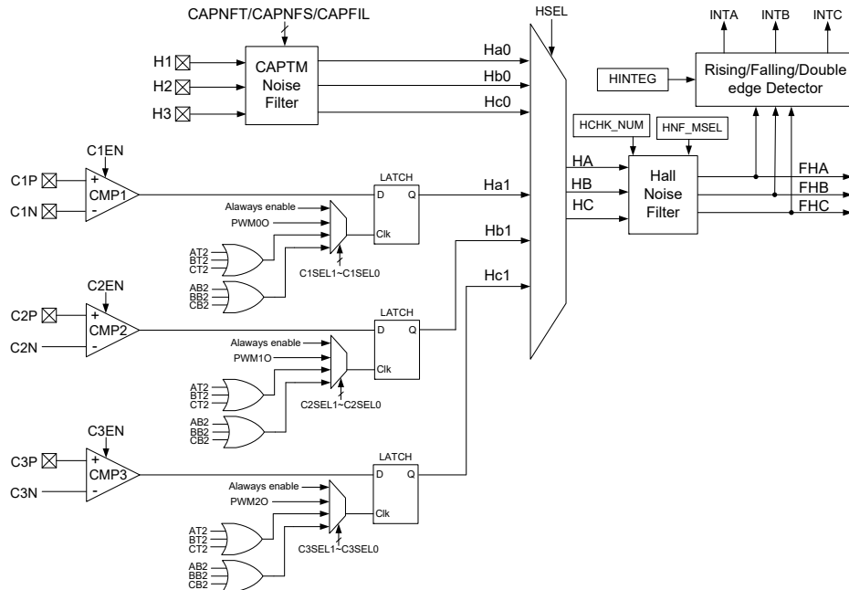
Hall Sensor Noise Filter Block Diagram
