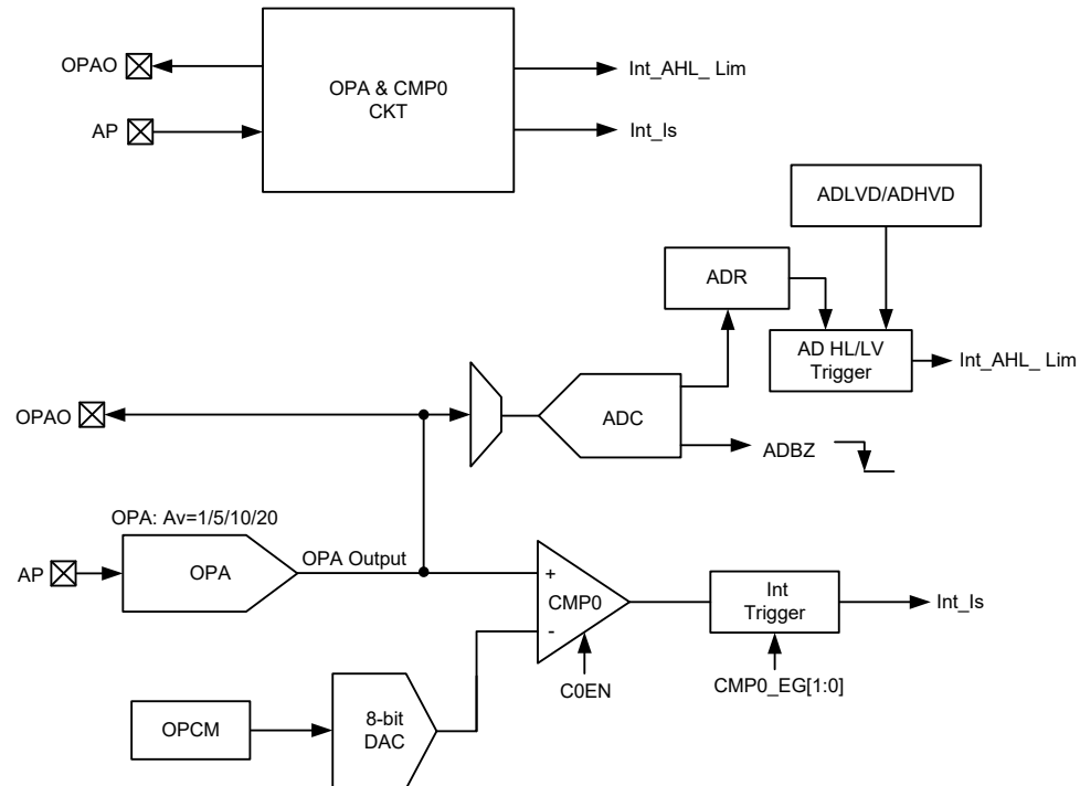
Over Current Detector Block Diagram
