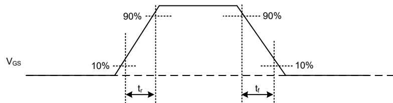
Gate Voltage ( V_{GS} ) Rising Time ( t_r ) and Falling Time ( t_f )
