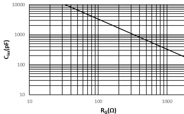
C_{iss} and R_G Curve
