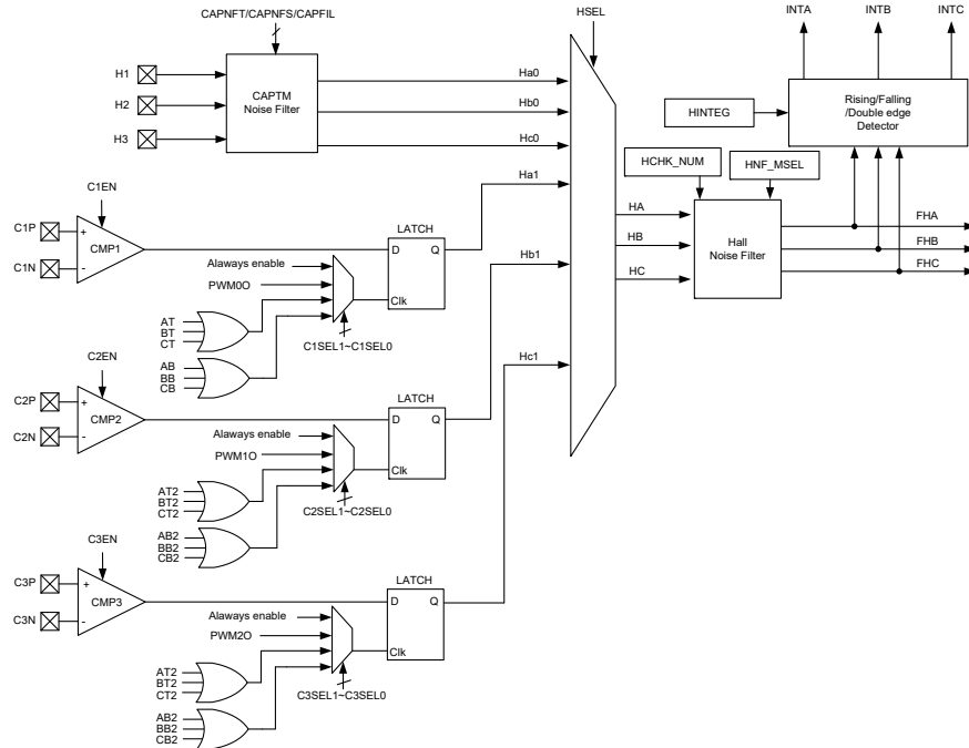
Hall Sensor Noise Filter Block Diagram
