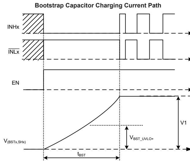
Bootstrap Capacitor Charging Time ( t_{BST} )
