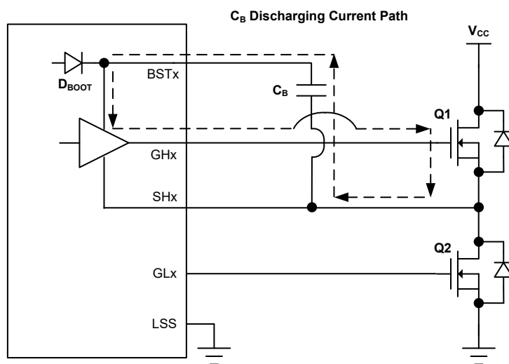
Bootstrap Capacitor ( C_B ) Discharging Current Path
