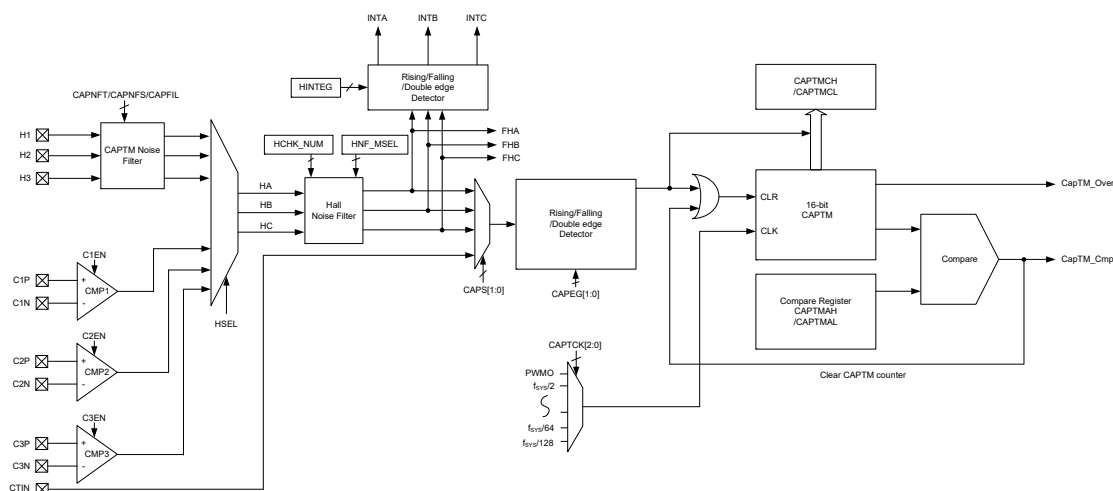
Capture Timer Block Diagram
