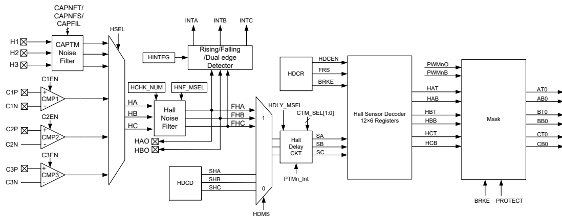
Hall Sensor Decoder Block Diagram
