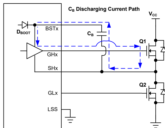
Bootstrap Capacitor ( C_B ) Discharging Current Path
