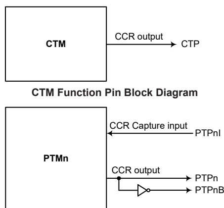
PTMn Function Pin Block Diagram (n=0~1)
