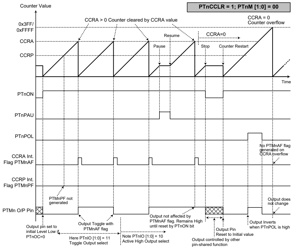
Compare Match Output Mode – PTnCCLR=1 (n=0~3)
