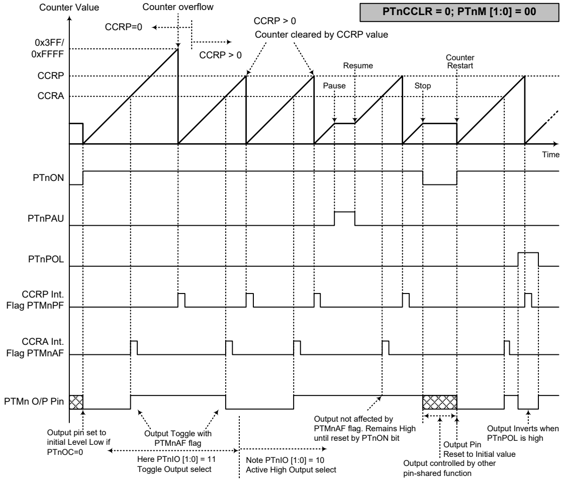
Compare Match Output Mode – PTnCCLR=0 (n=0~3)
