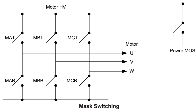
Mask Function Block Diagram
