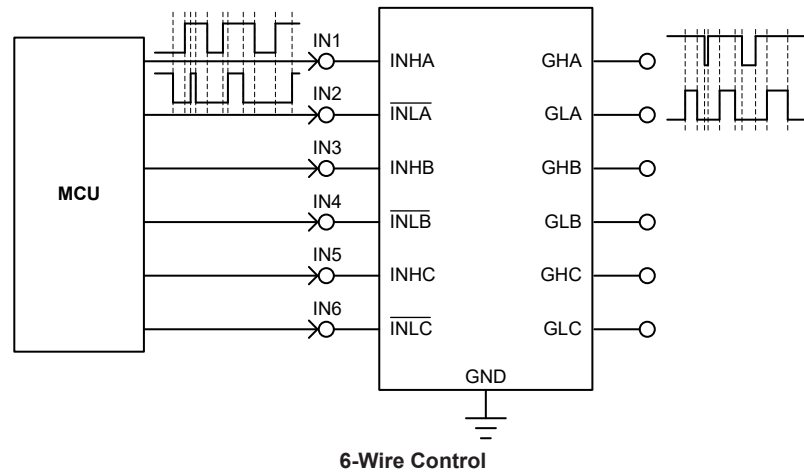
6-Wire Control
