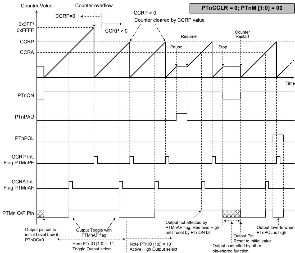
Compare Match Output Mode – PTnCCLR=0 ( n=0\sim3 )
