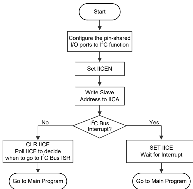
I 2 C Bus Initialisation Flowchart
