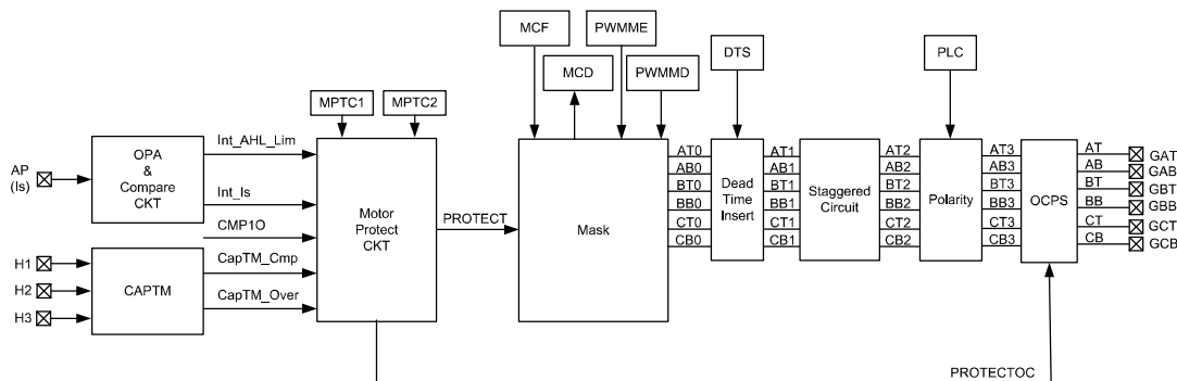
Motor Protection Function Block Diagram
