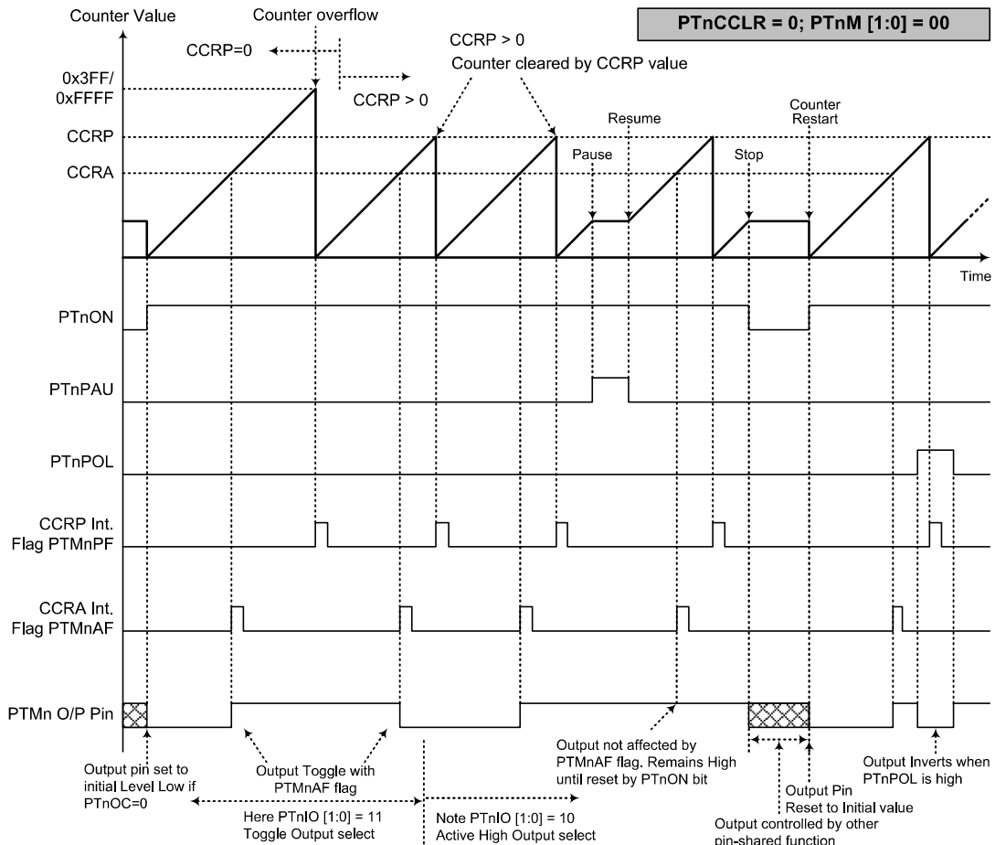
Compare Match Output Mode – PTnCCLR=0 (n=0~3)
