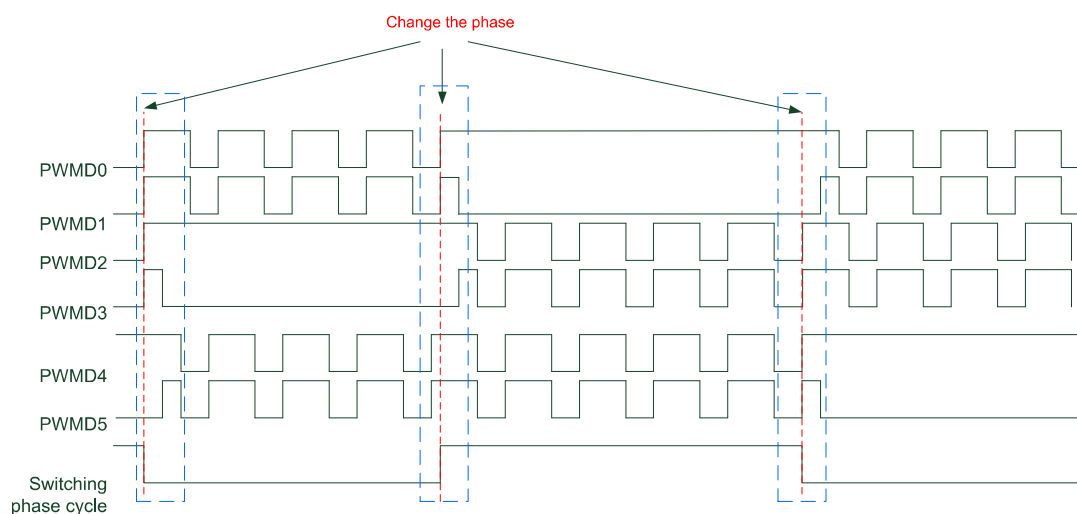
Phase Change Timing – PWMEDO=0
