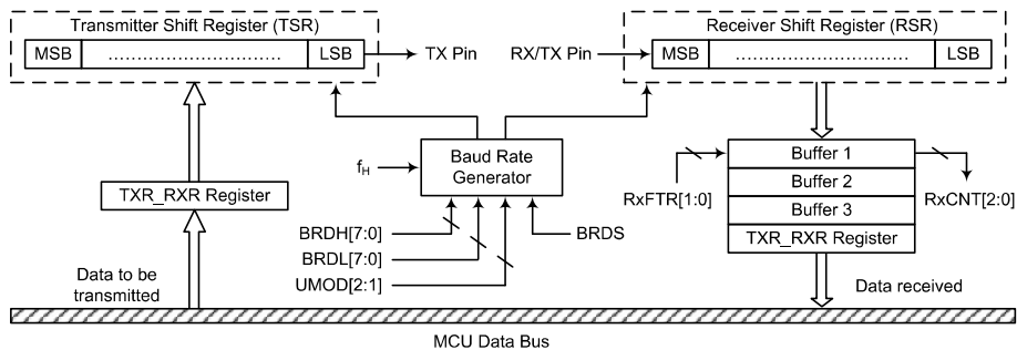
UART Data Transfer Block Diagram – SWM=0
