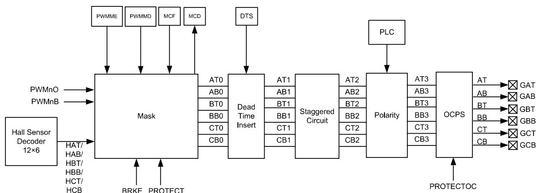
Mask Function Block Diagram
