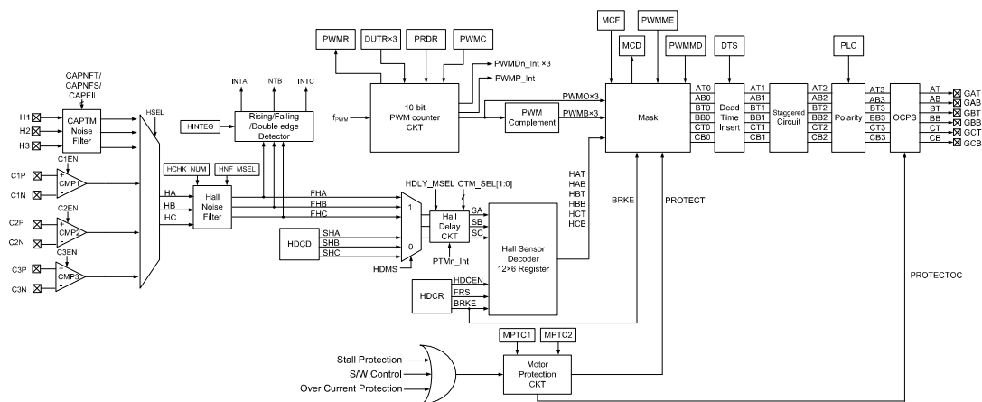
BLDC Motor Control Block Diagram
