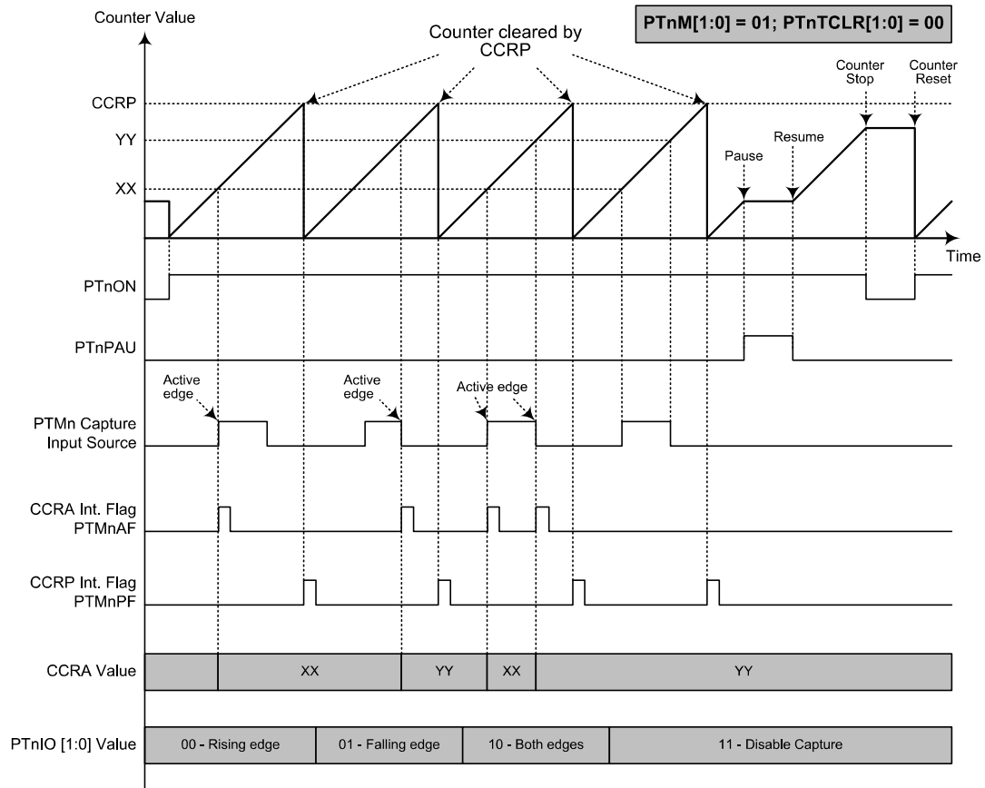
Capture Input Mode – PTnTCLR[1:0]=00 (n=0)
