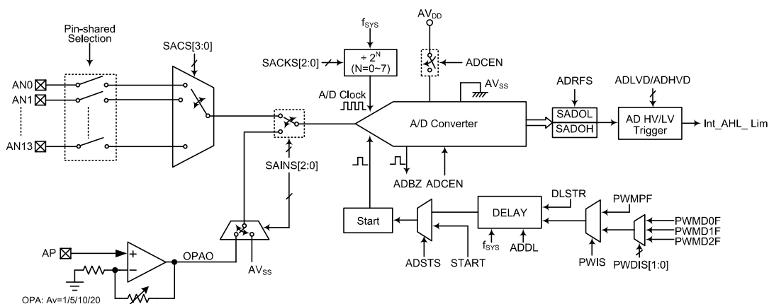
A/D Converter Structure
