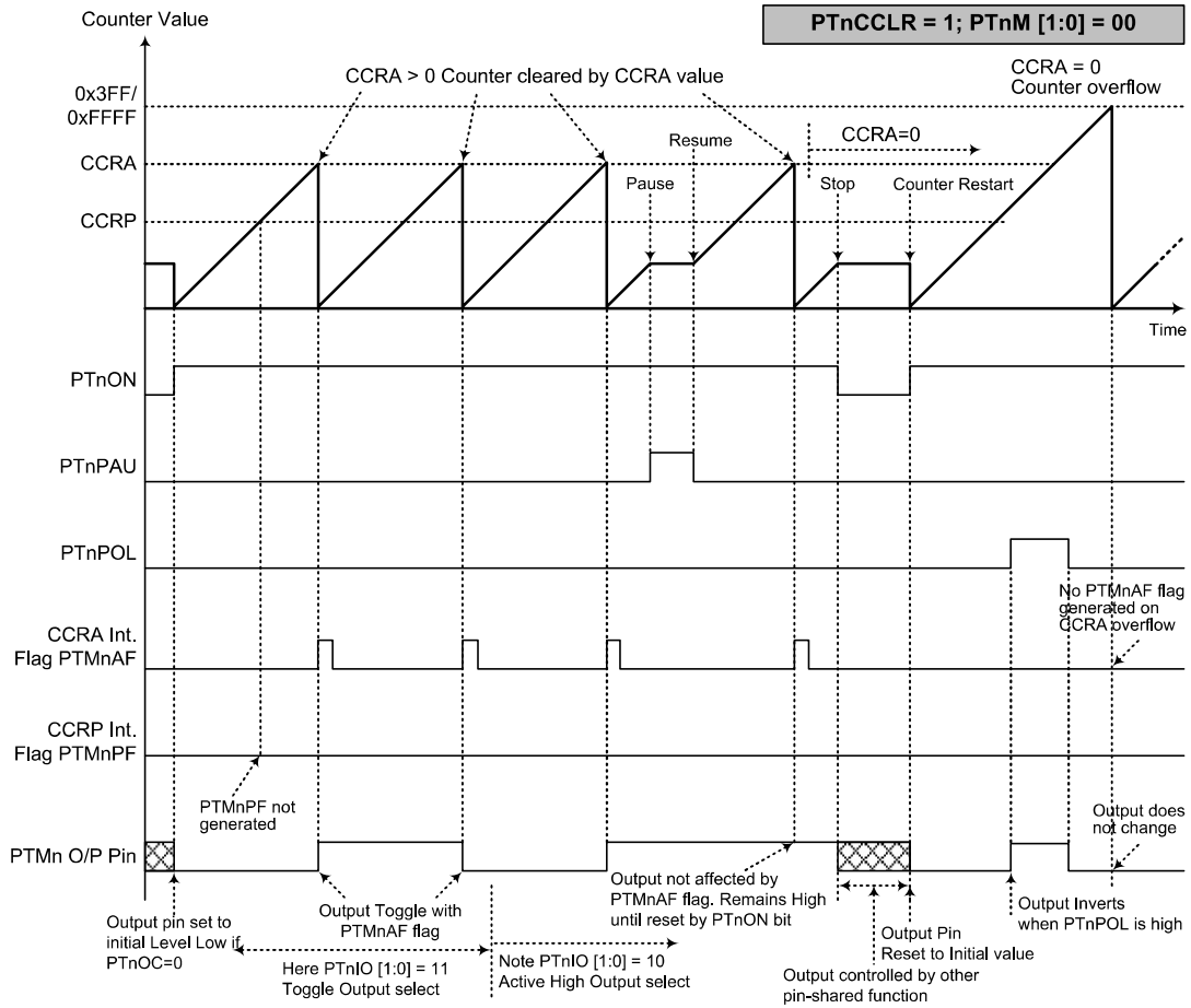
Compare Match Output Mode – PTnCCLR=1 (n=0~3)
