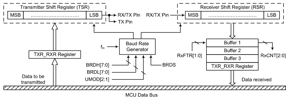
UART Data Transfer Block Diagram – SWM=1
