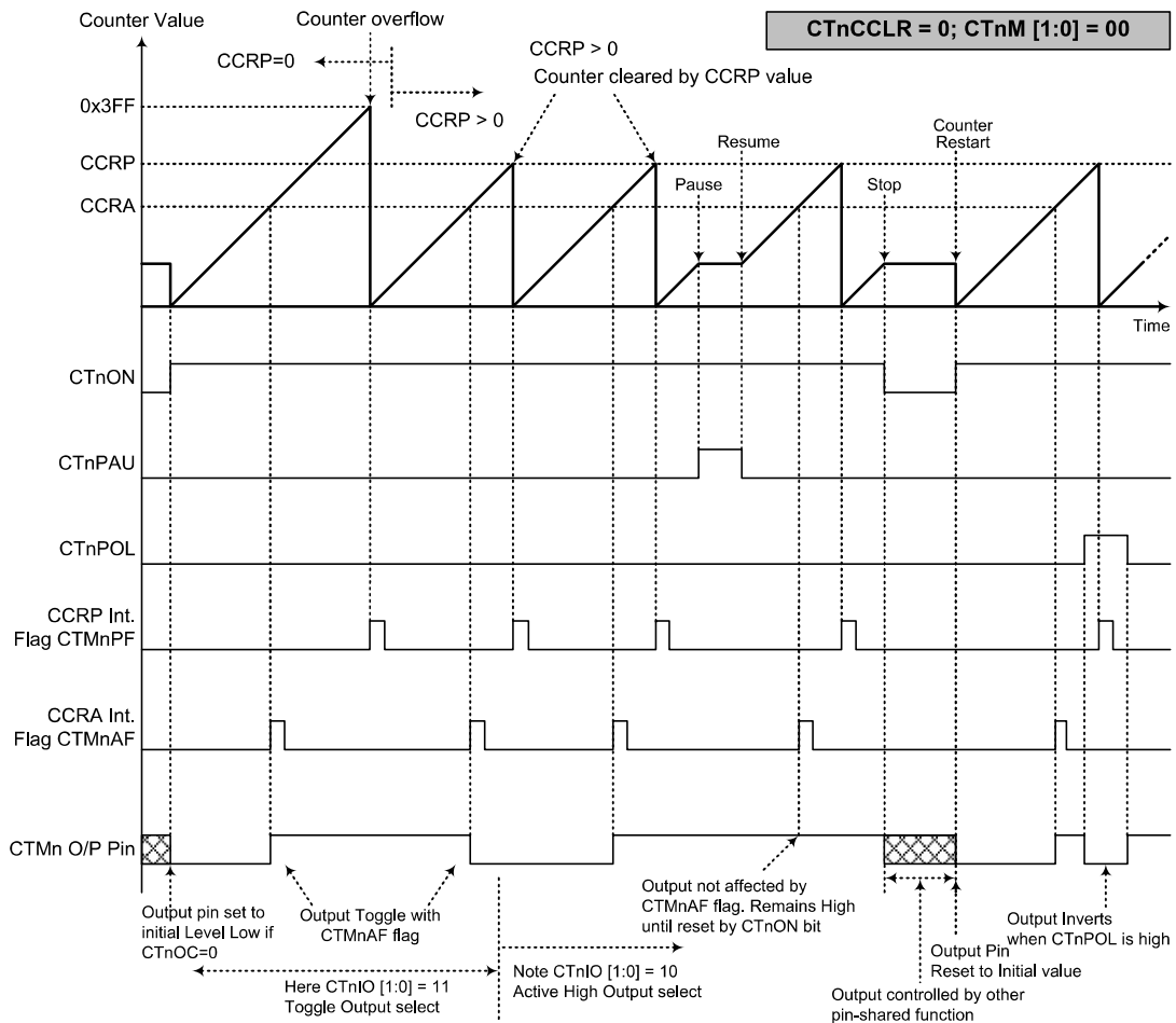
Compare Match Output Mode – CTnCCR=0 (n=0~1)
