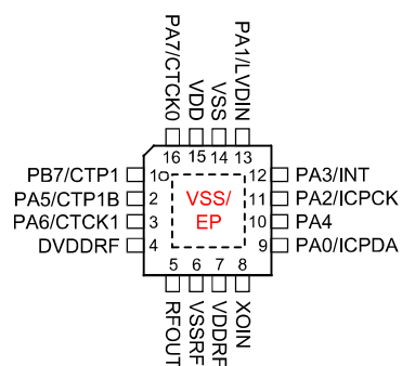
BC68F3132 16 QFN-A
