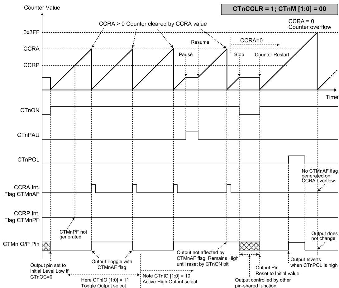
Compare Match Output Mode – CTnCCR=1 (n=0~1)
