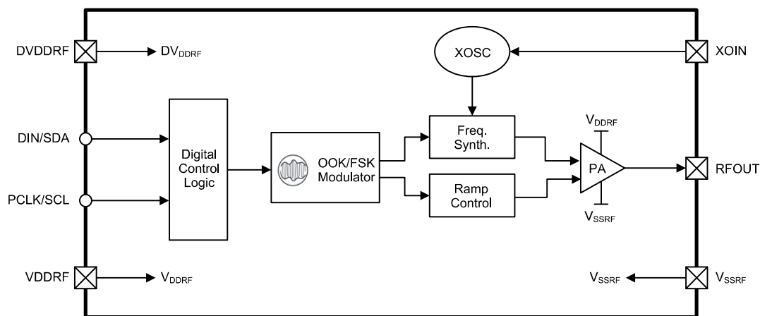
RF Transmitter Block Diagram
