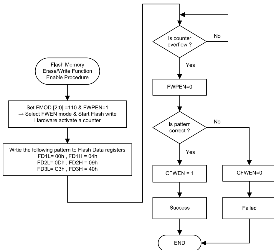
Flash Memory Erase/Write Function Enable Procedure
