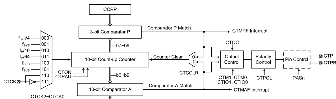
Compact Type TM Block Diagram
