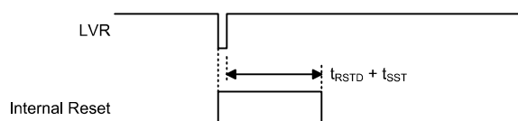
Low Voltage Reset Timing Chart
