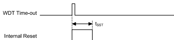
Watchdog Time-out Reset during SLEEP or IDLE Mode Timing Chart
