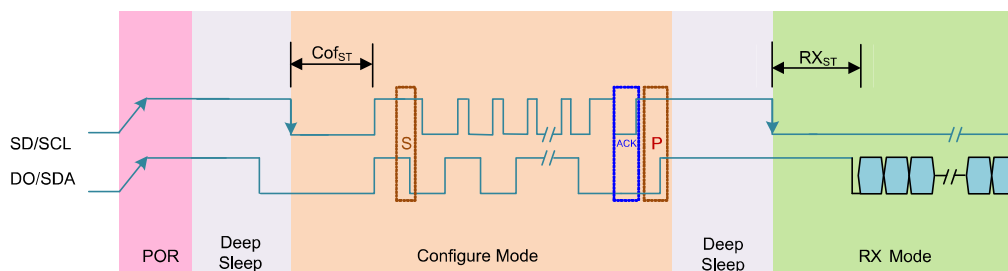
Entering and Leaving Configuration Mode Timing Diagram
