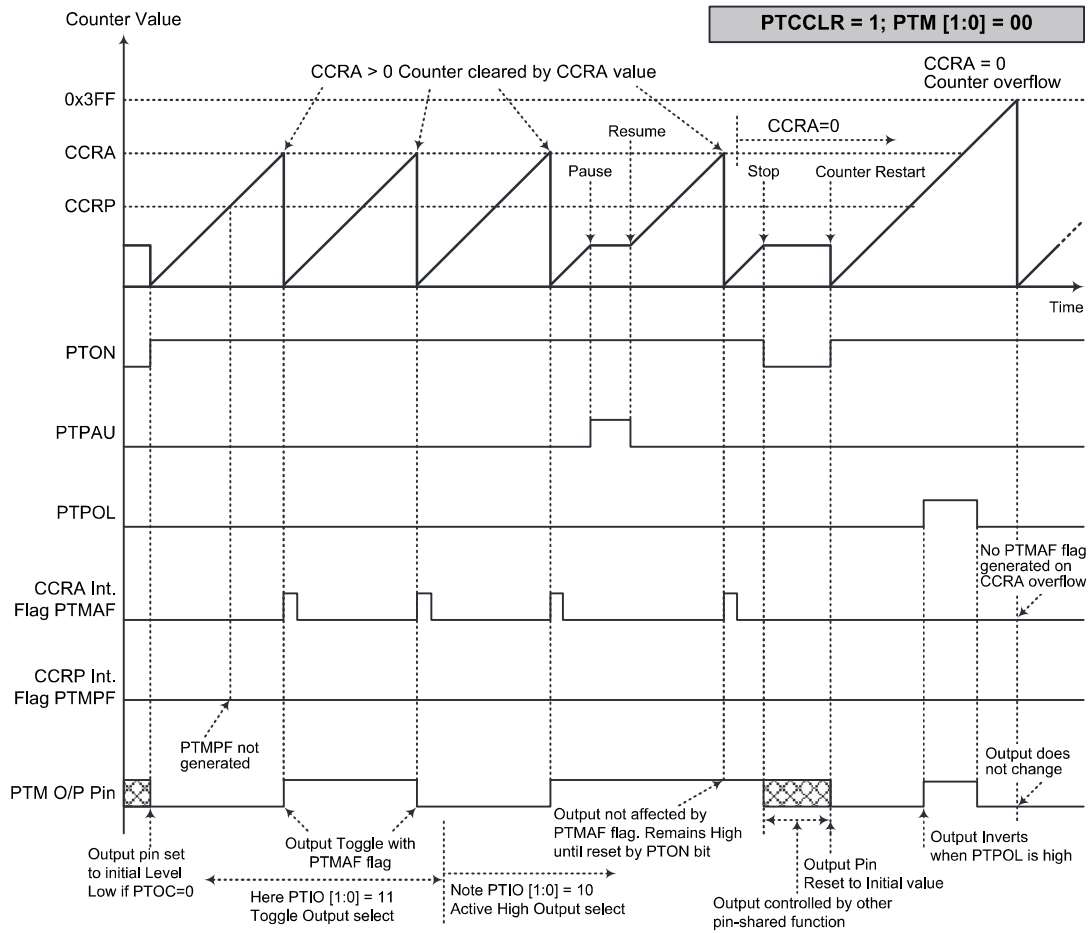
Compare Match Output Mode – PTCCLR=1
