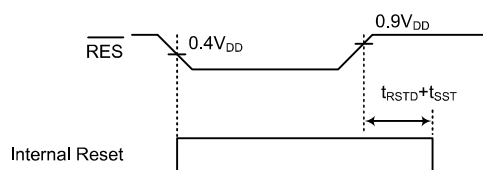
RES Reset Timing Chart
