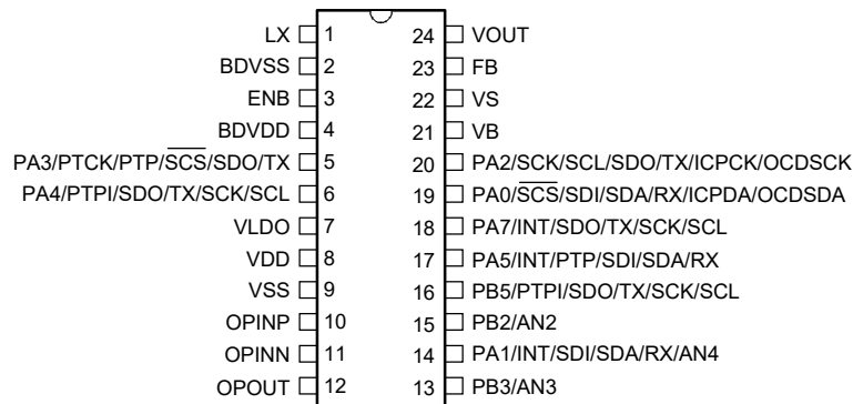
BA45F6830/BA45V6830 24 SSOP-A
