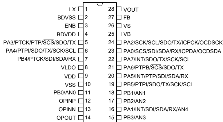
BA45F6830/BA45V6830 28 SSOP-A
