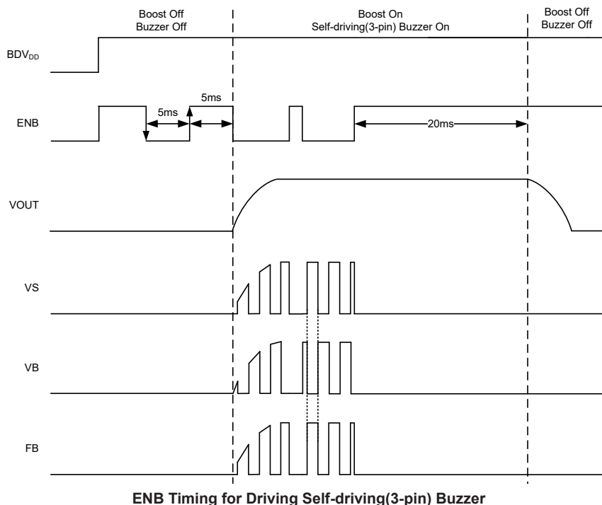
ENB Timing for Driving Self-driving(3-pin) Buzzer
