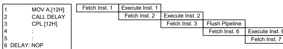
Instruction Fetching
