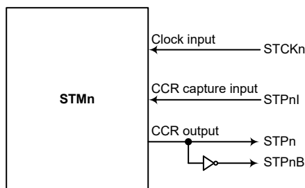
STM Function Pin Block Diagram (n=0~1)
