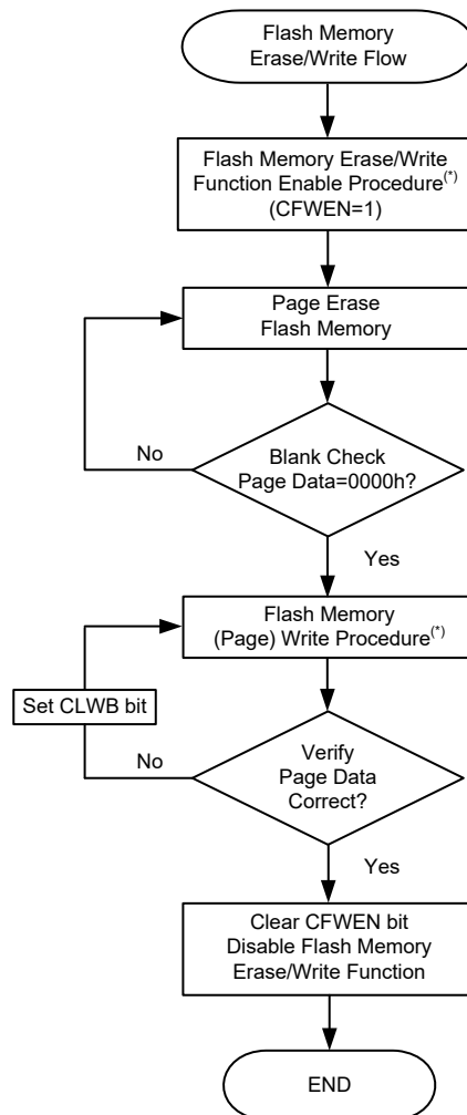
Flash Memory Erase/Write Flow
