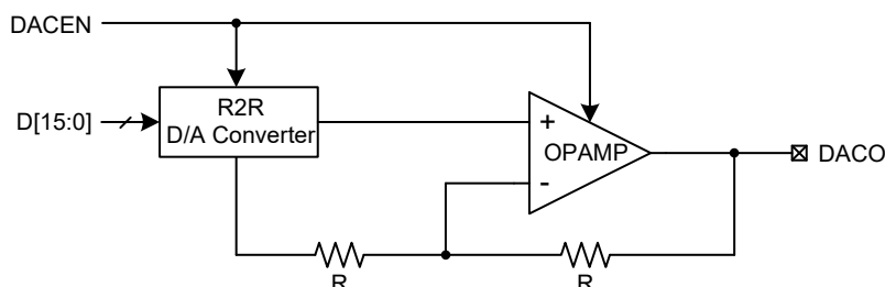
16-bit D/A Converter Block Diagram
