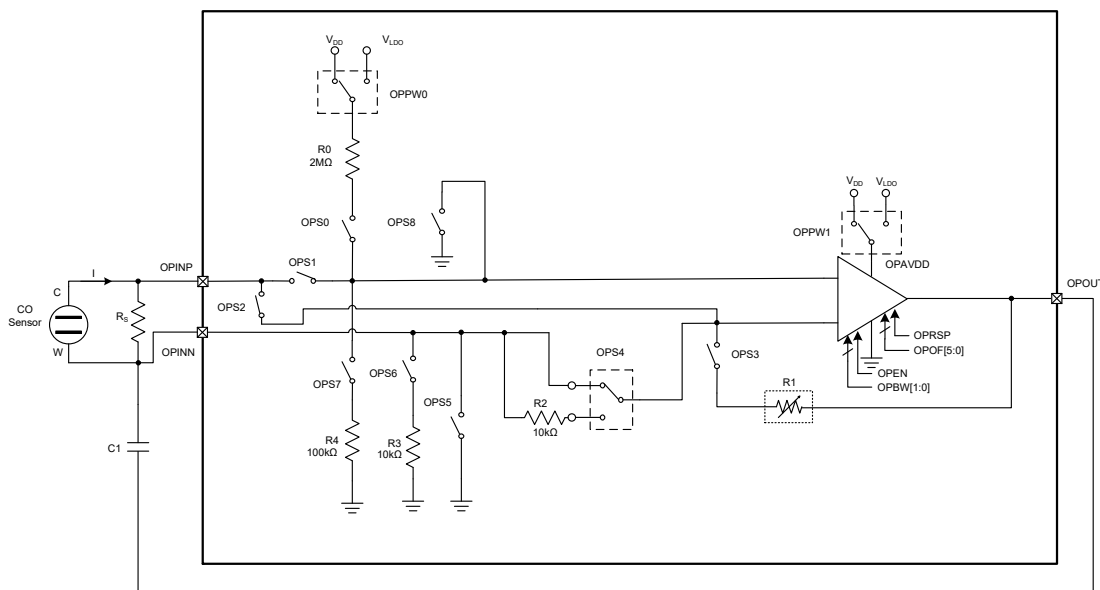
CO/Gas Detector Application Schematic
