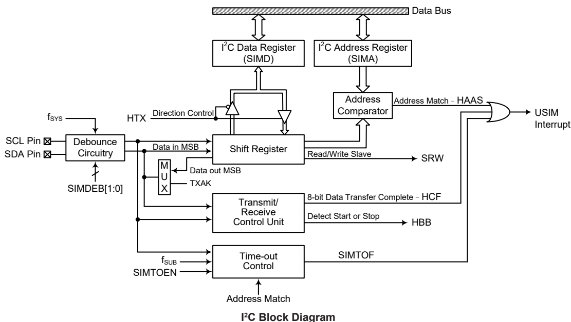
I²C Block Diagram
