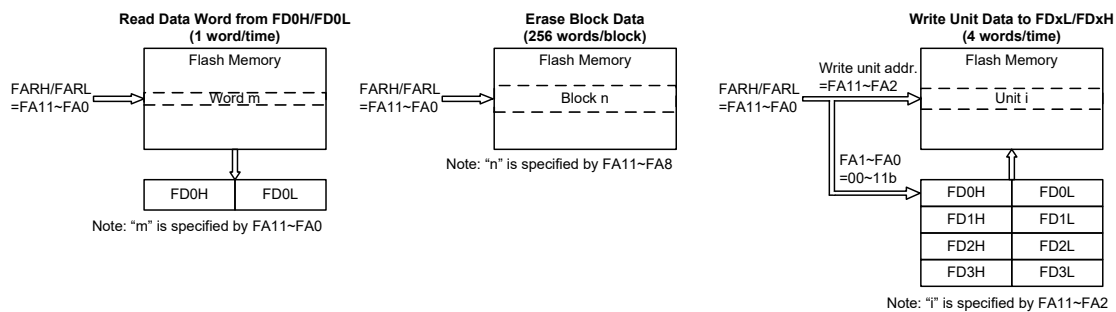
Flash Memory IAP Read/Erased/Write Structure
