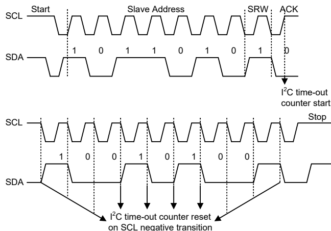
I²C Time-out
