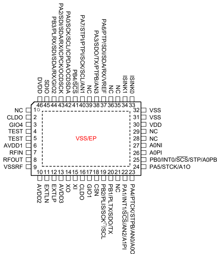
BA45F5640 BA45V5640 46 QFN-A
