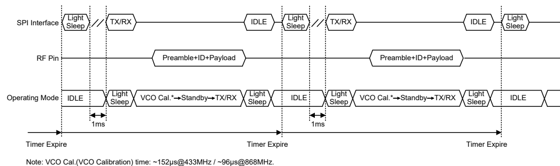
Periodical TX/RX Timing
