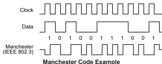
Manchester Code Example
