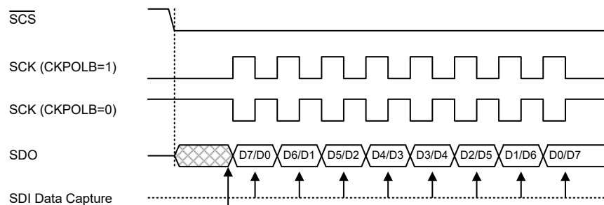
SPI Slave Mode Timing – CKEG=0 (SDO does not change until first SCK edge)
