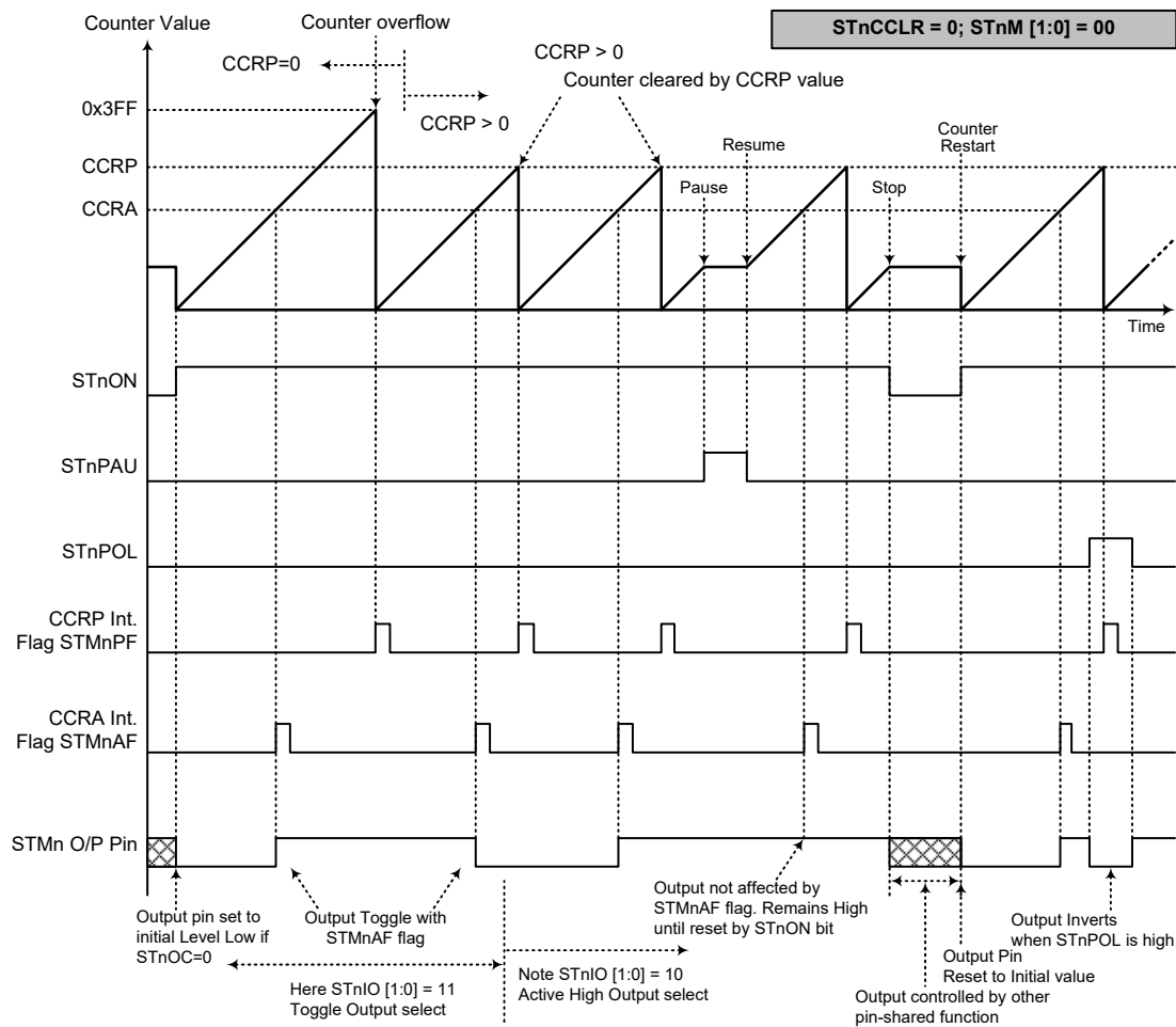
Compare Match Output Mode – STnCCLR=0 ( n=0\sim1 )
