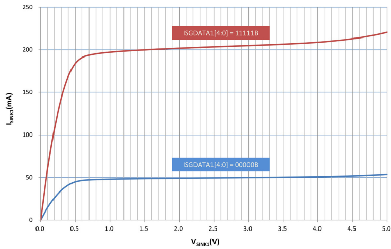
V_SINK1 VS. I_SINK1 I_SINK1 Characteristic Curve
