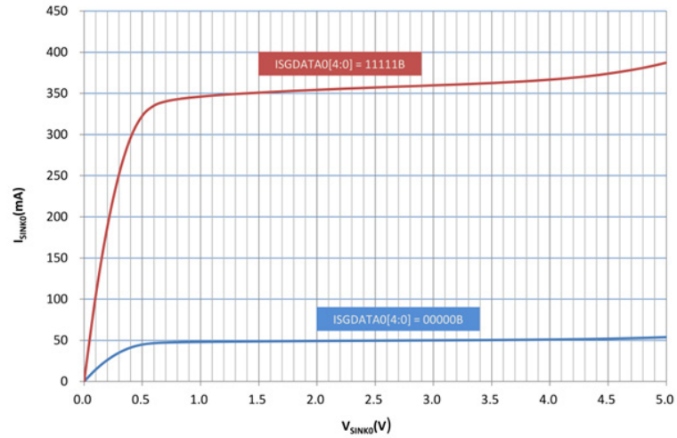
V_SINK0 VS. I_SINK0 I_SINK0 Characteristic Curve
