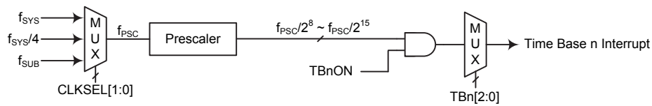
Time Base Interrupt (n=0 or 1)
