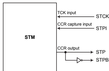
STM Function Block Diagram
