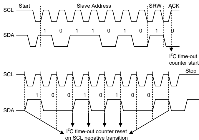
I²C Time-out
