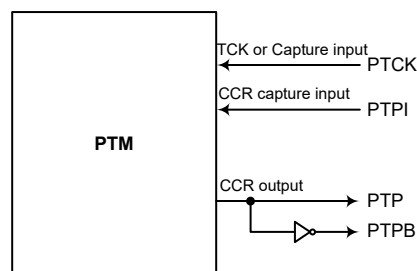
PTM Function Block Diagram
