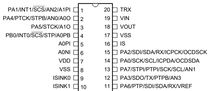
BA45F5542/BA45V5542 20 SSOP-A
