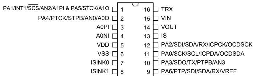
BA45F5542-2/BA45V5542-2 16 NSOP-A
