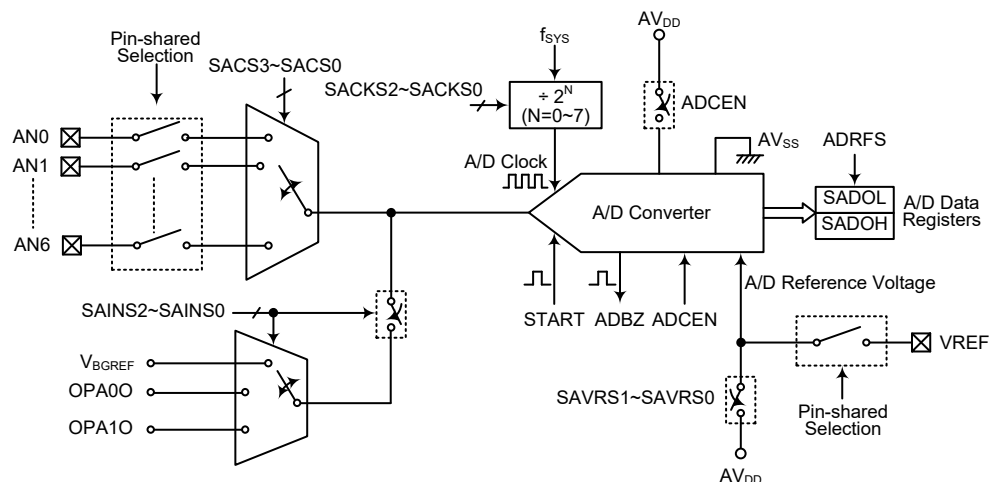
A/D Converter Structure
