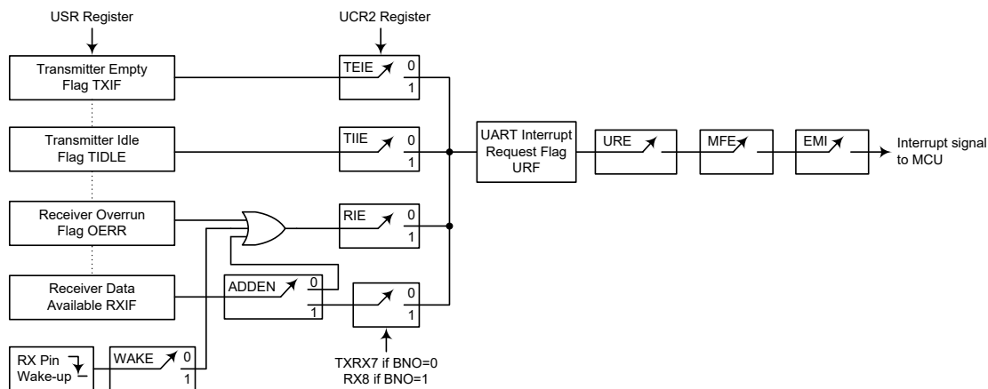
UART Interrupt Structure
