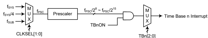
Time Base Interrupt (n=0 or 1)
