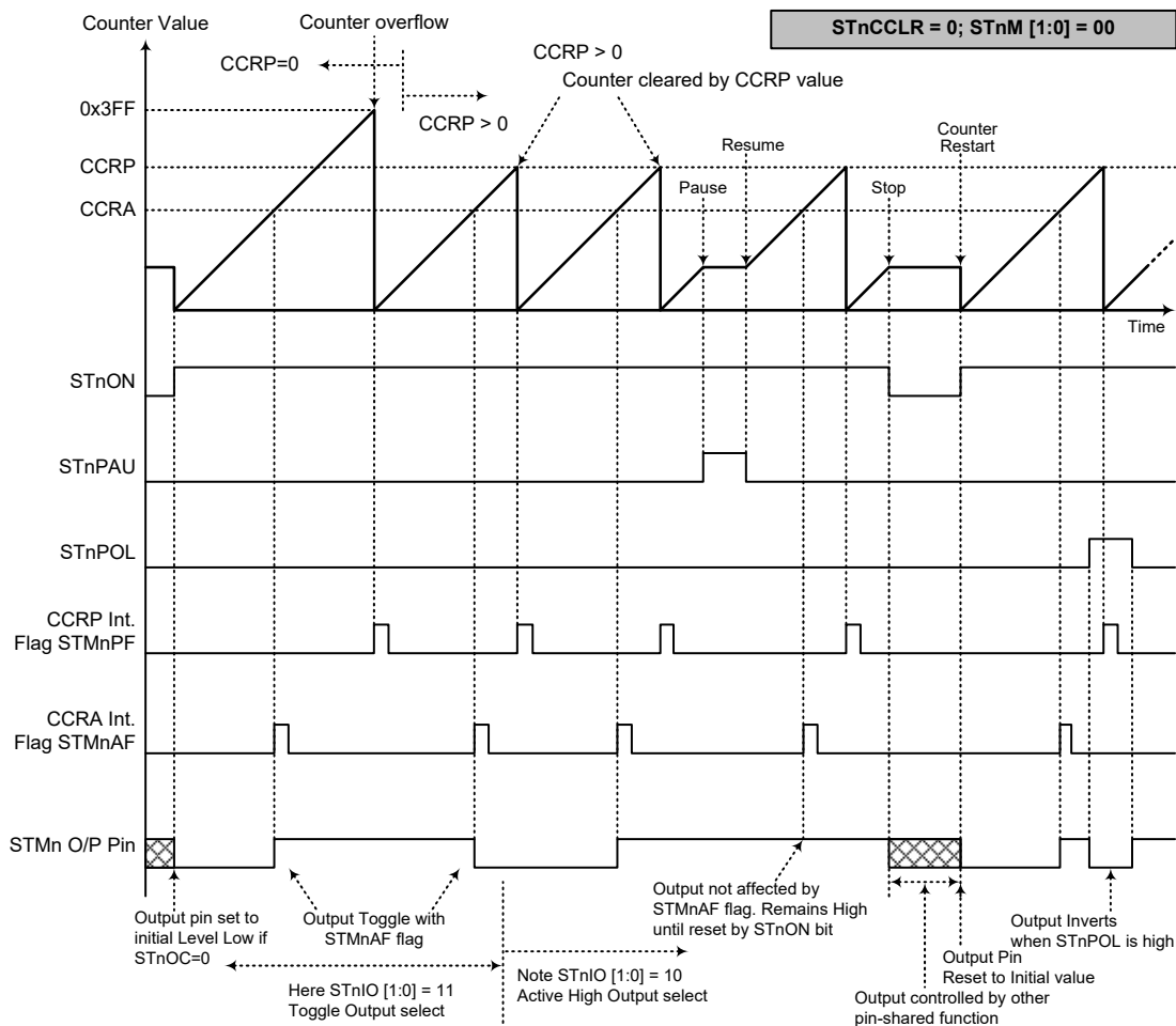
Compare Match Output Mode – STnCCLR=0 (n=0~1)
