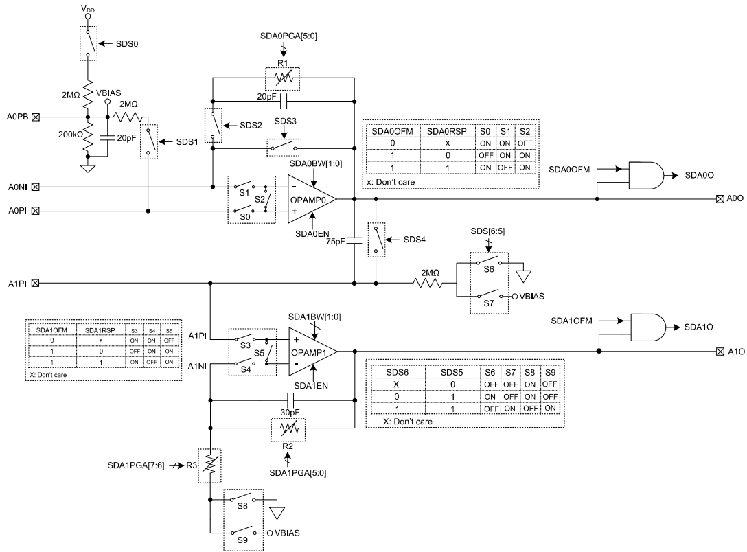
Smoke Detector AFE Block Diagram
