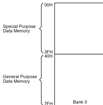
Data Memory Structure
