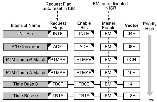
Interrupt Structure
