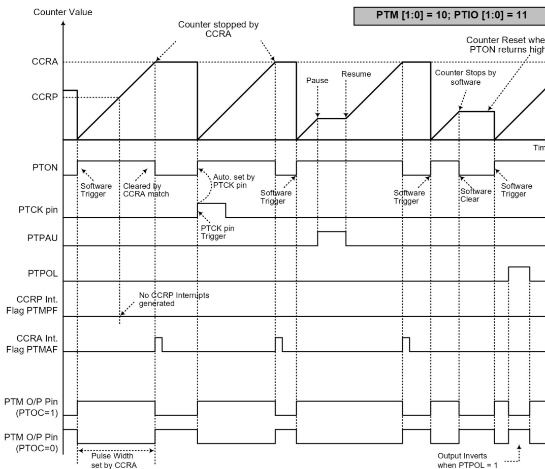
Single Pulse Output Mode
