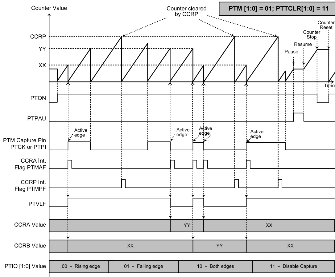
Capture Input Mode – PTnTCLR[1:0] = 11
