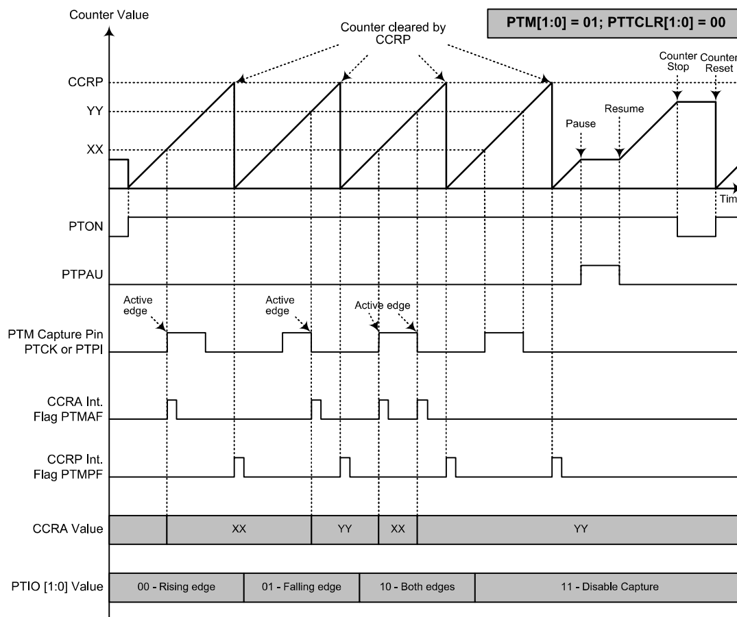
Capture Input Mode – PTTCLR[1:0]=00
