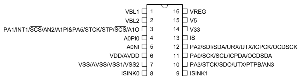
BA45F25543/BA45V25543 16 NSOP-A
