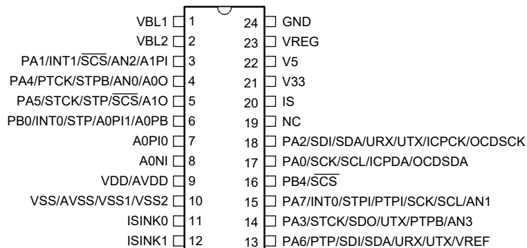
BA45F25543/BA45V25543 24 SSOP-A
