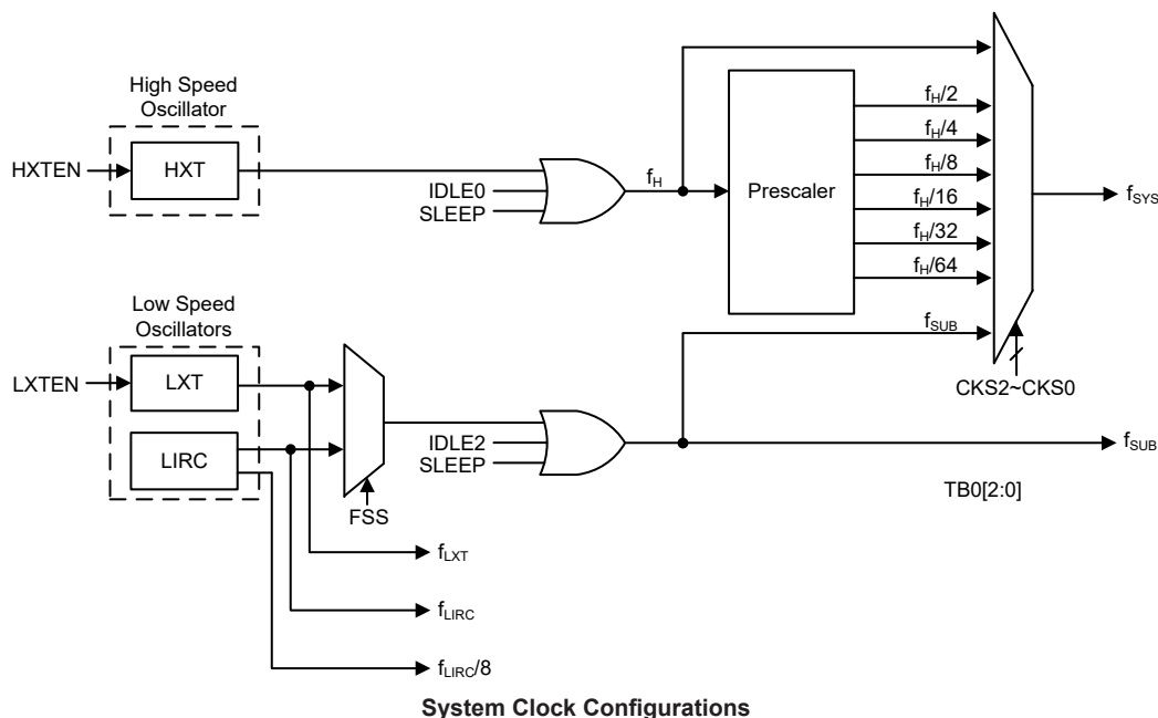
System Clock Configurations
