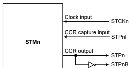
TM External Pins
